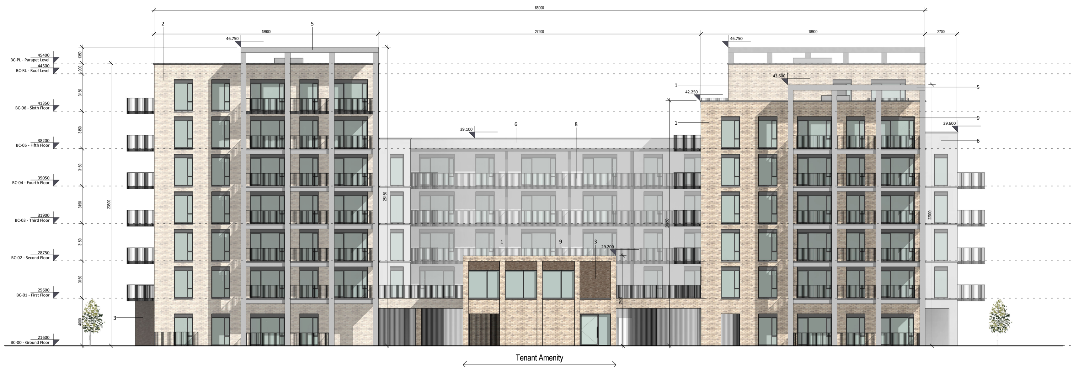
1 BC East Elevation 1:200
